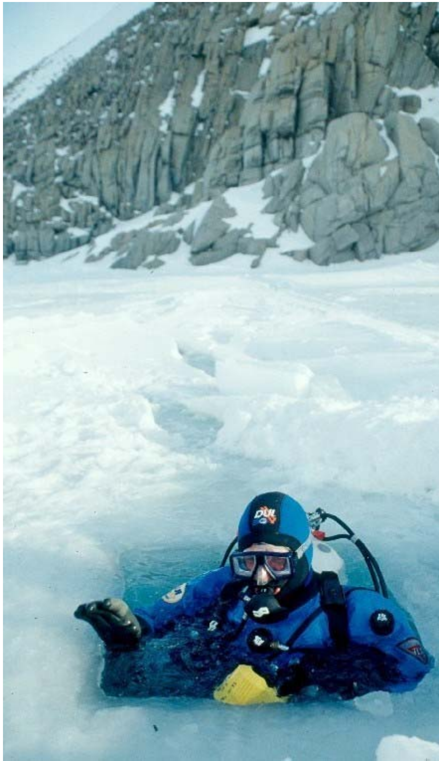
Couloir Cliffs, Antarctica
